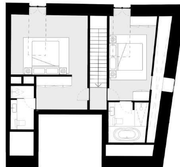
PISO 3 floor 3
