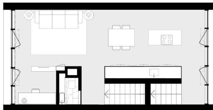
PISO 1 floor 1
