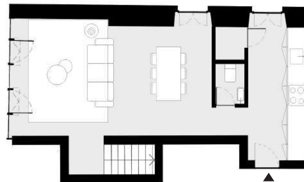
PISO 2 floor 2
