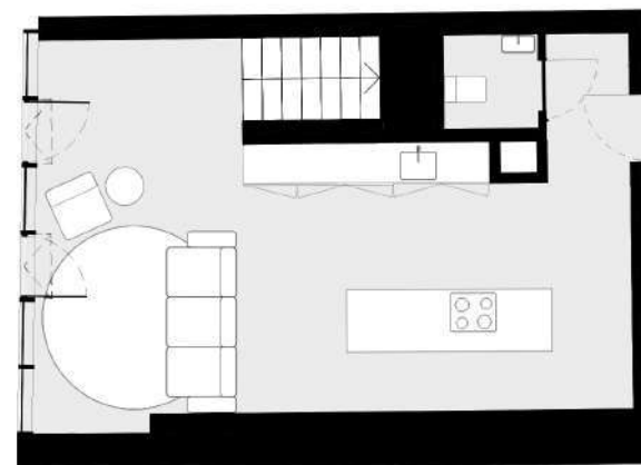
PISO 1 floor 1
