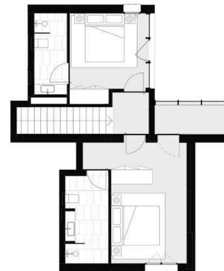
PISO 1 floor 1
