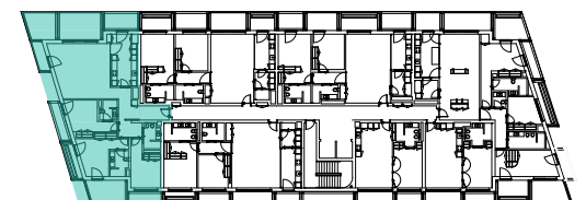
PLANTA PISO 3 THIRD FLOOR
