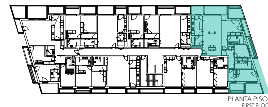
PLANTA PISO 1 FIRST FLOOR
