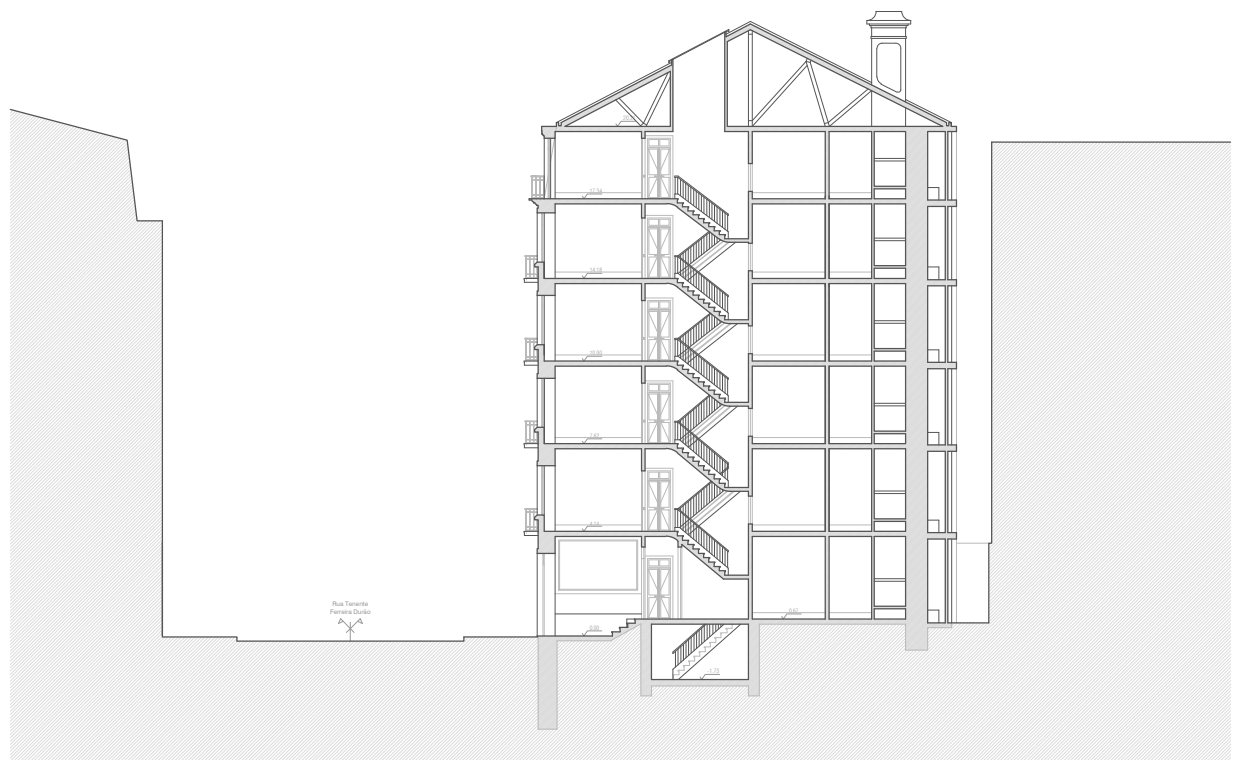
SECTION BB'
